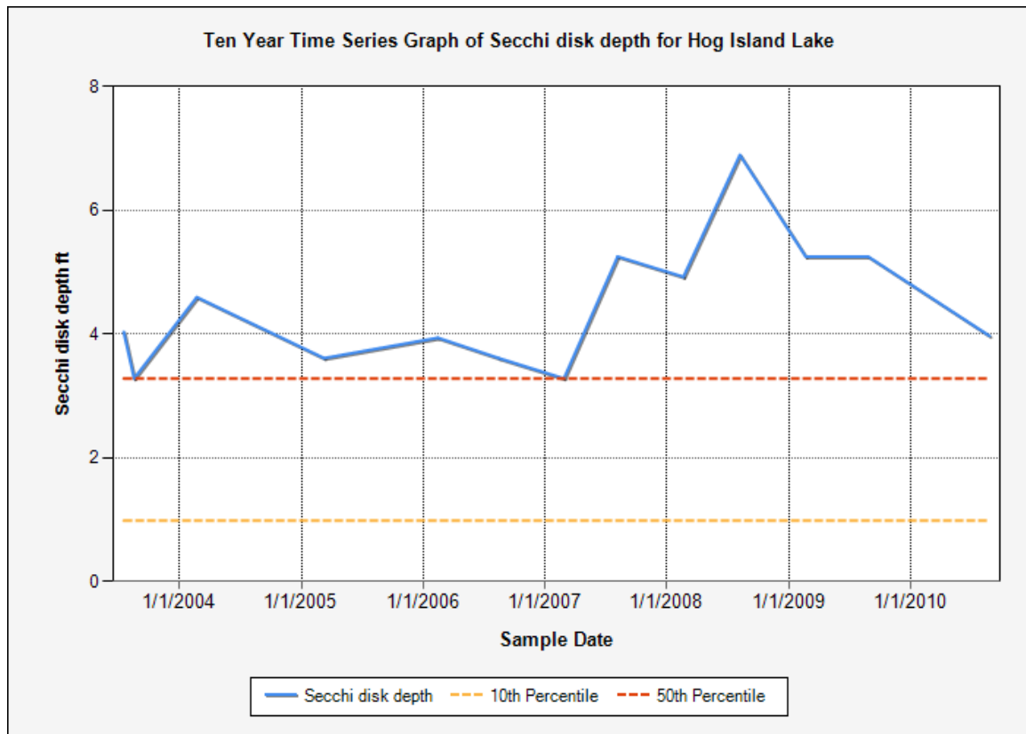
Figure 9. Recent Secchi Disk graph for Hog Island Lake viii
