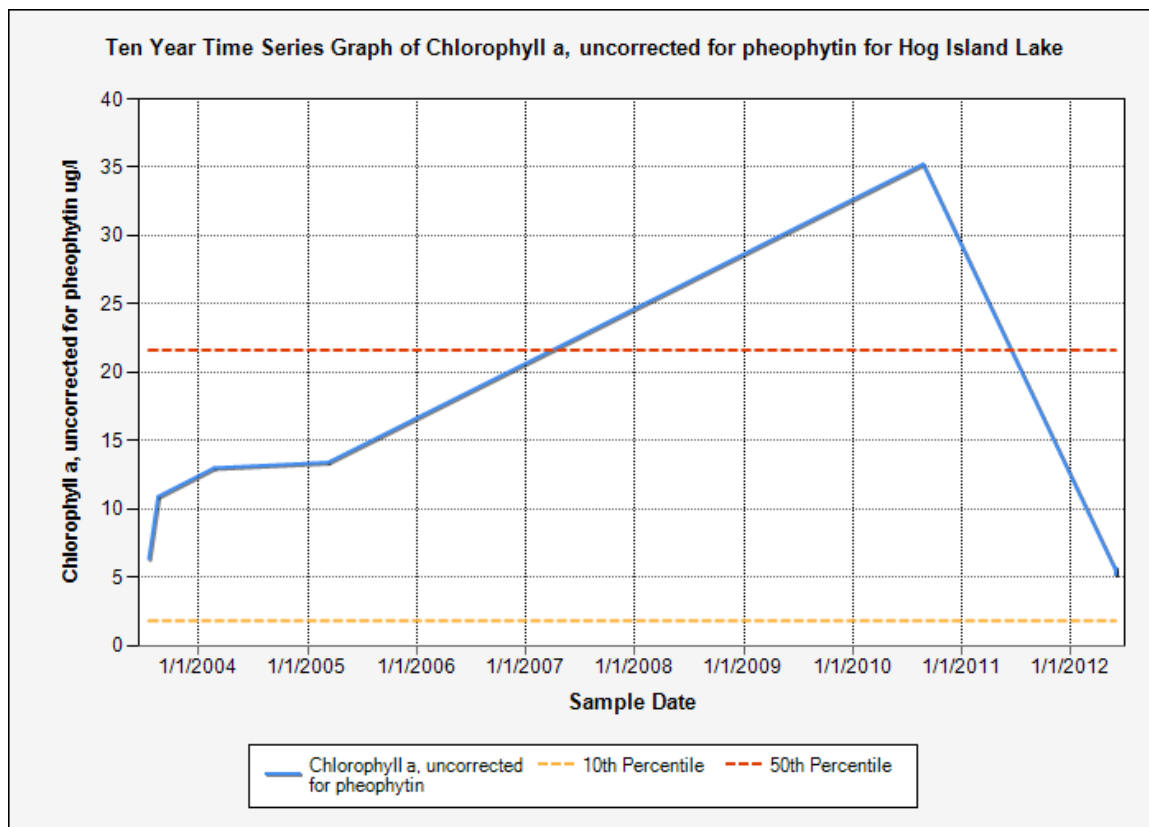
Figure 8. Recent Chlorophyll a graph for Hog Island Lake vii
