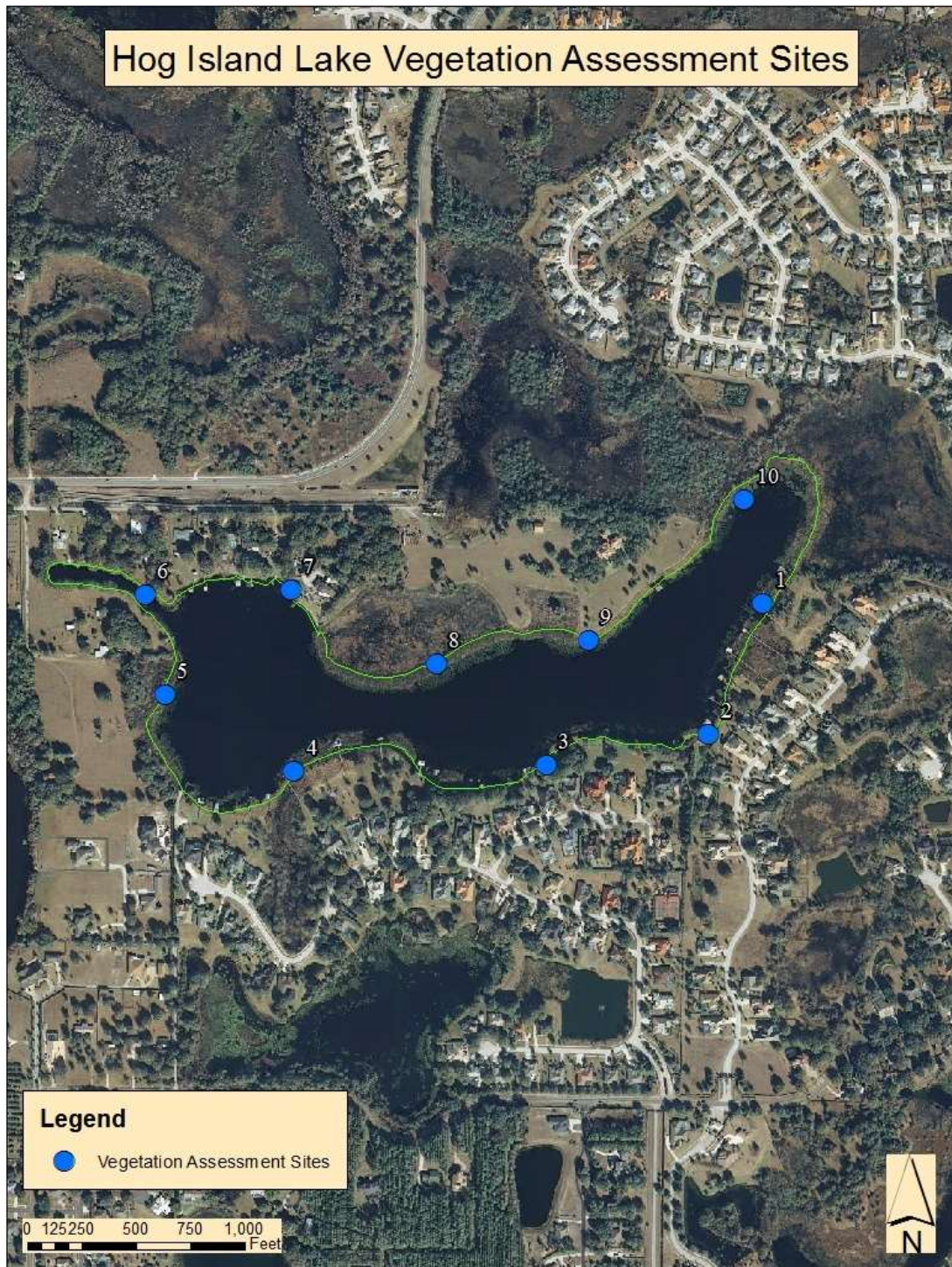
Figure 3. Vegetation assessment site map for Hog Island Lake for 2012.
