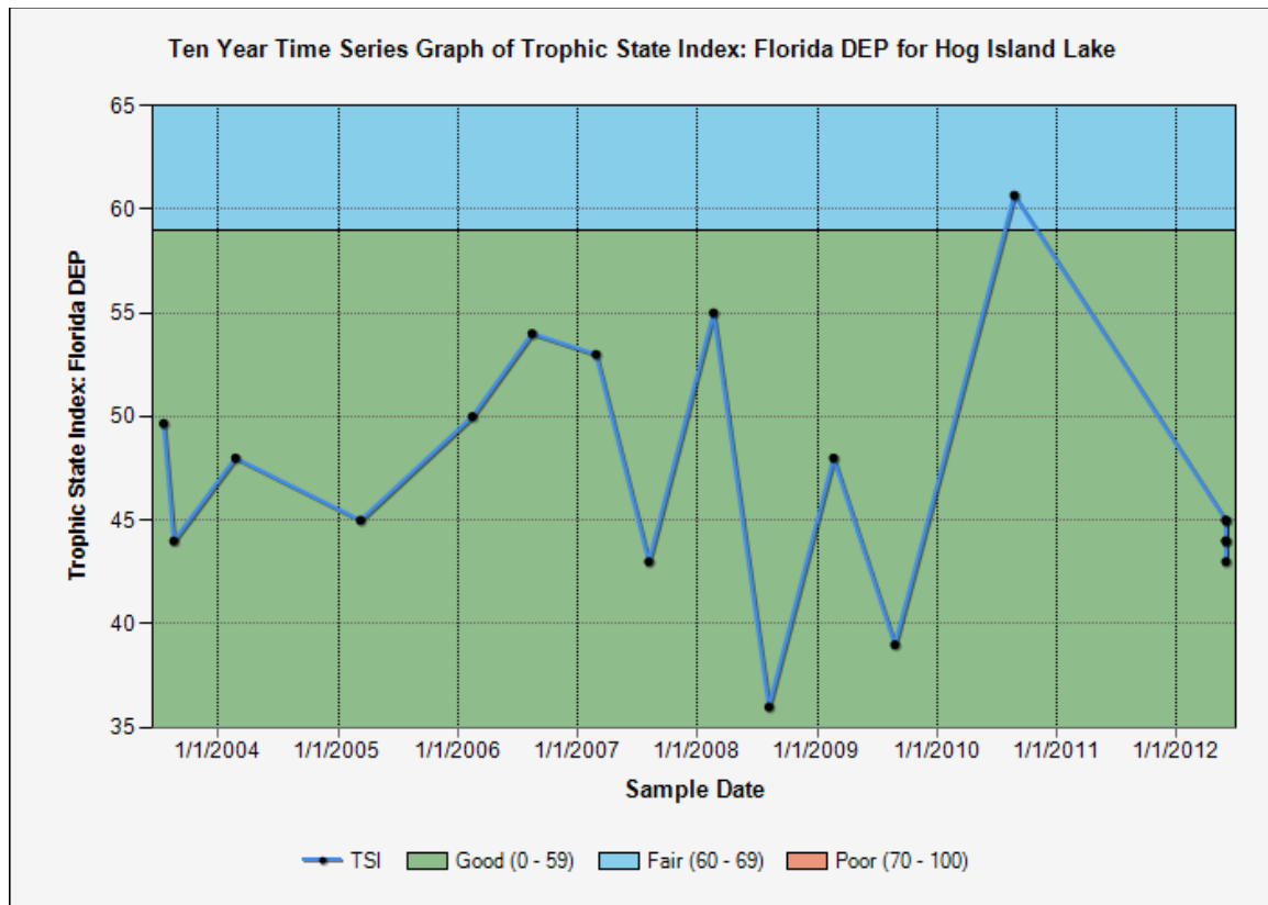
Figure 7. Recent Trophic State Index (TSI) graph for Hog Island Lake vi
