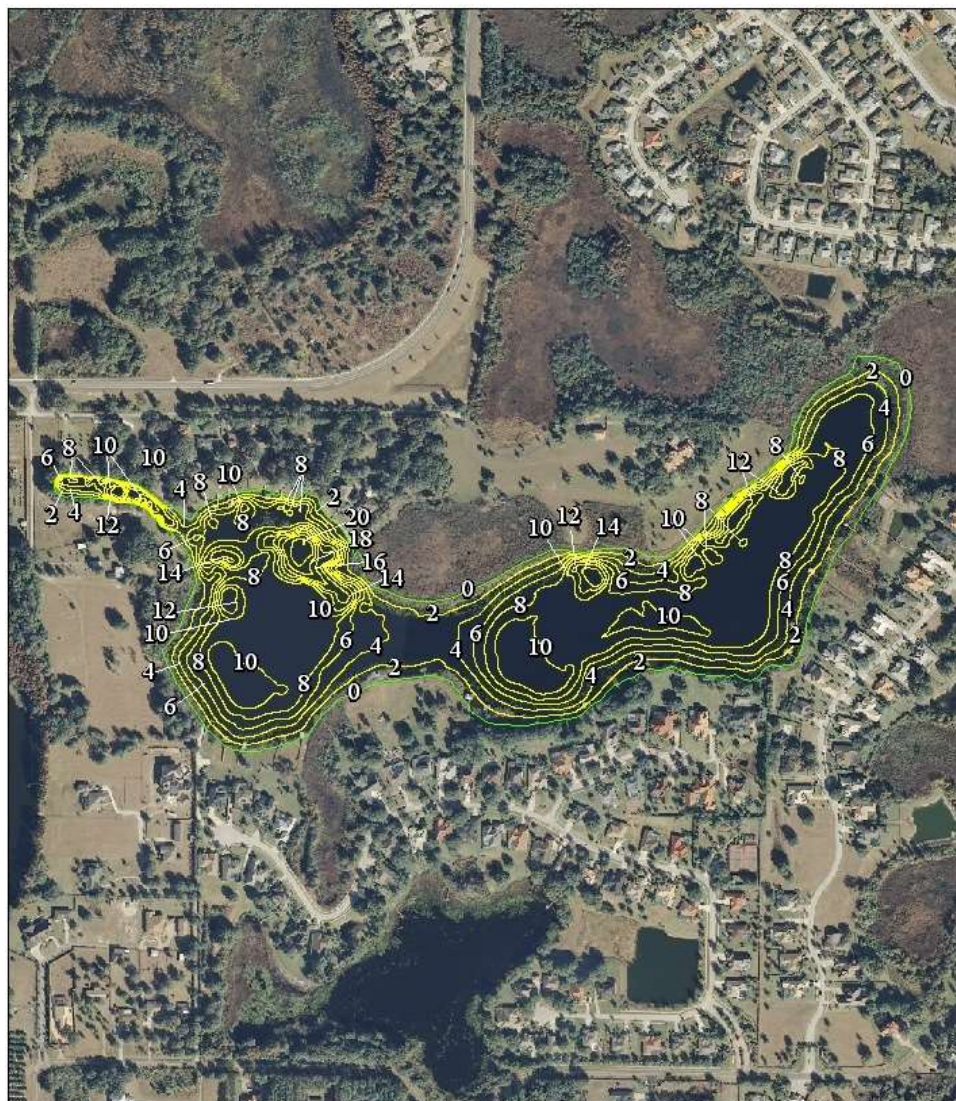
Figure 2. Hog Island Lake 2-Foot Bathymetric Contour Map created from data collected during the 2012 lake assessment.
